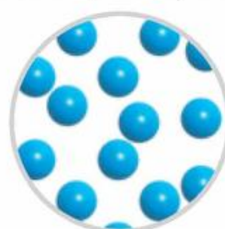
ciecz
