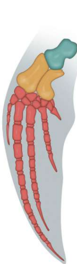
waleń
