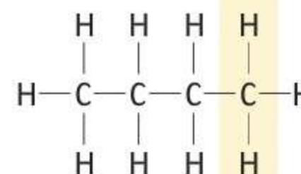
butan C_4H_{10}
