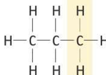
propan C_3H_8
