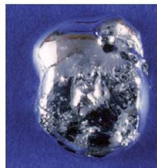
gal Ga
